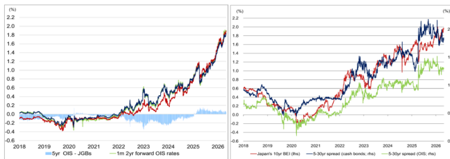
Fig. 1: 5yr JGB yields and 5-30yr spread
